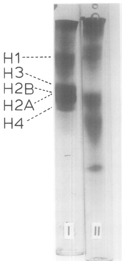
Figure 4. Gel electrophoresis patterns of calf thymus histones. Gel #I was obtained from SDS gel electrophoresis at pH 7.0, 8mA/tube for 4.5 hours. Gel #II was obtained from the two-stage method. SDS gel electrophoresis was carried out for first 2 hours and then the buffer was changed and electrophoresis was continued for 5.5 hours.
