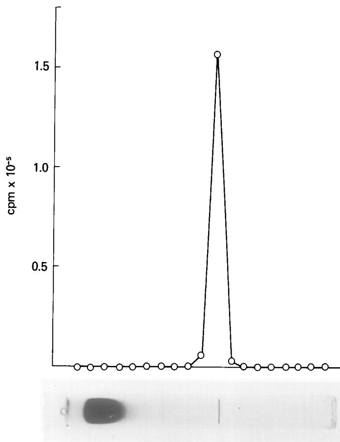
Figure 1. Electrophoresis of the b-TSH[ ^{35}\text{S} ] SDS complex at pH 9.5, 0.012 M sodium glycinate without SDS.
